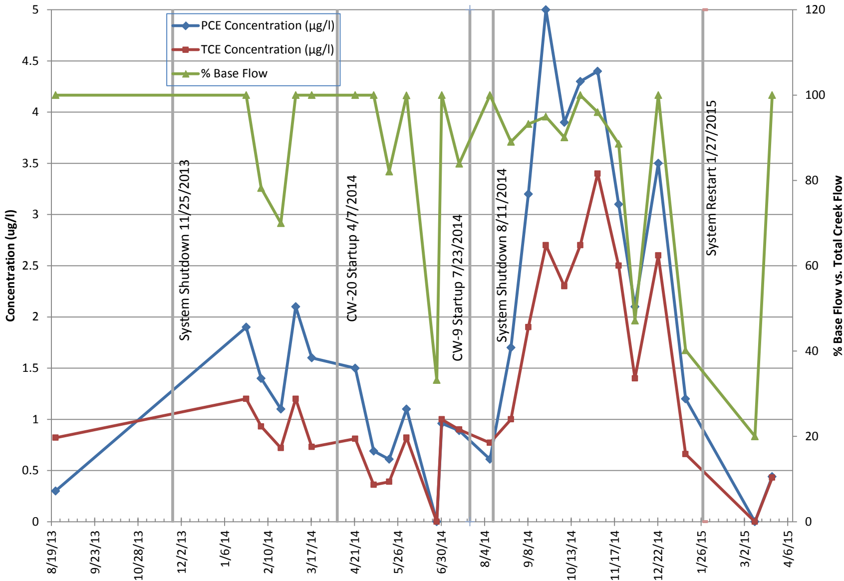
FIGURE 3.5-20 SW-13 Concentration vs Time compared to % Baseflow
